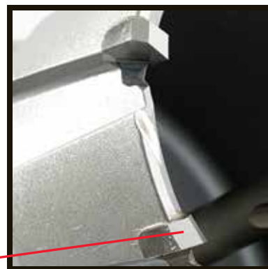
Triple Edge Tooth Geometry
